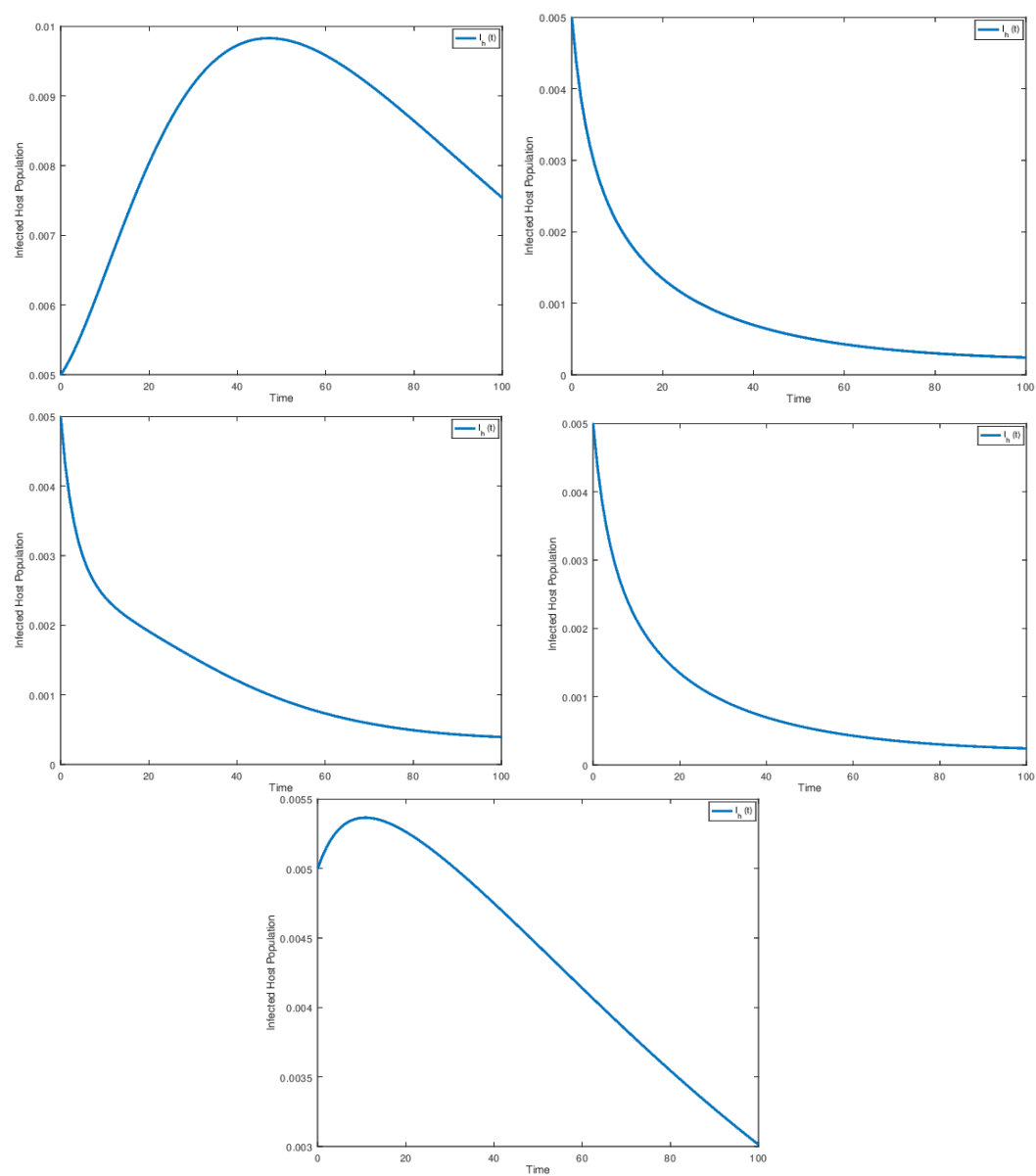
Figure 2: Infected Host Population
