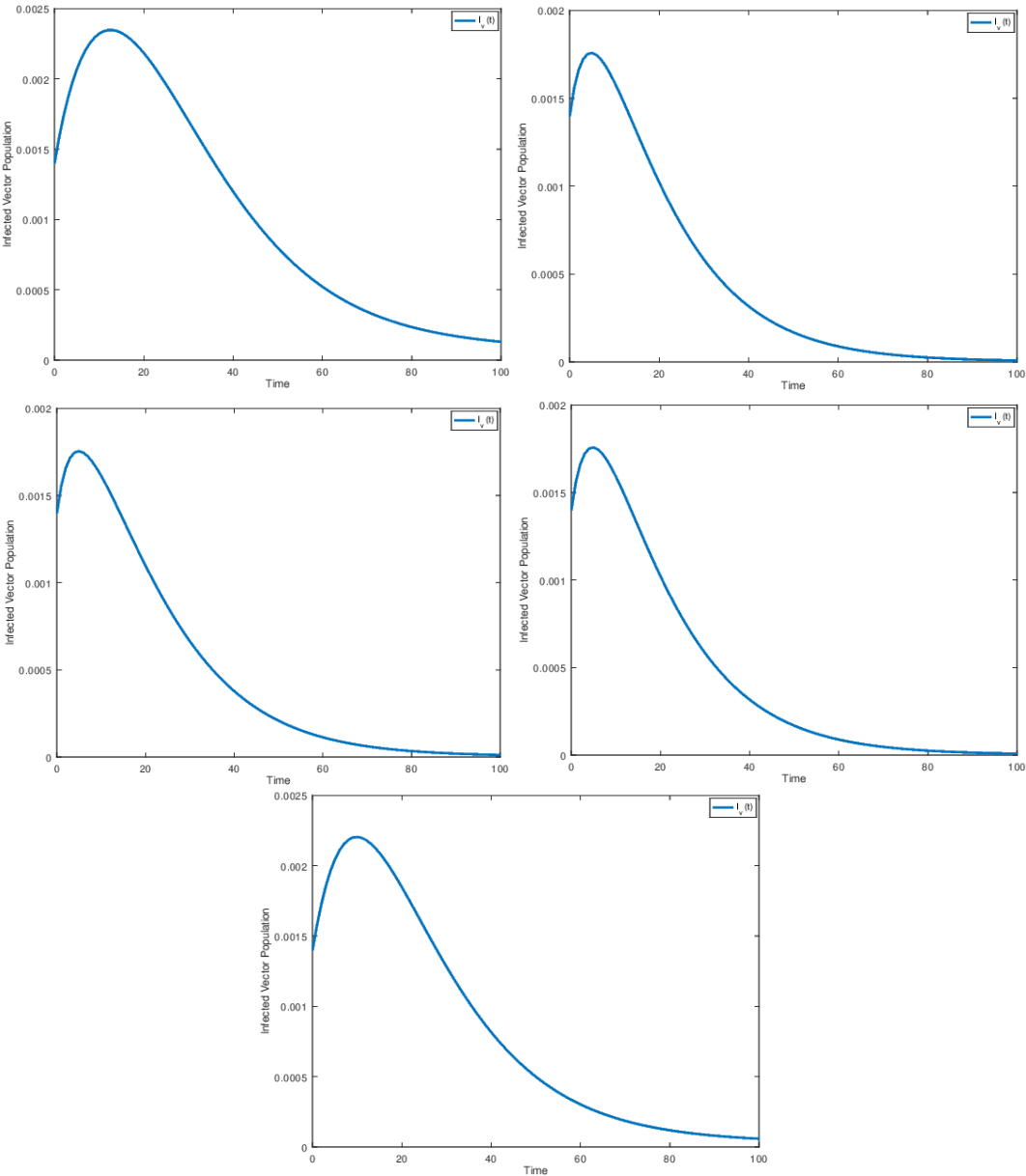
Figure 3: Infected Vector Population
