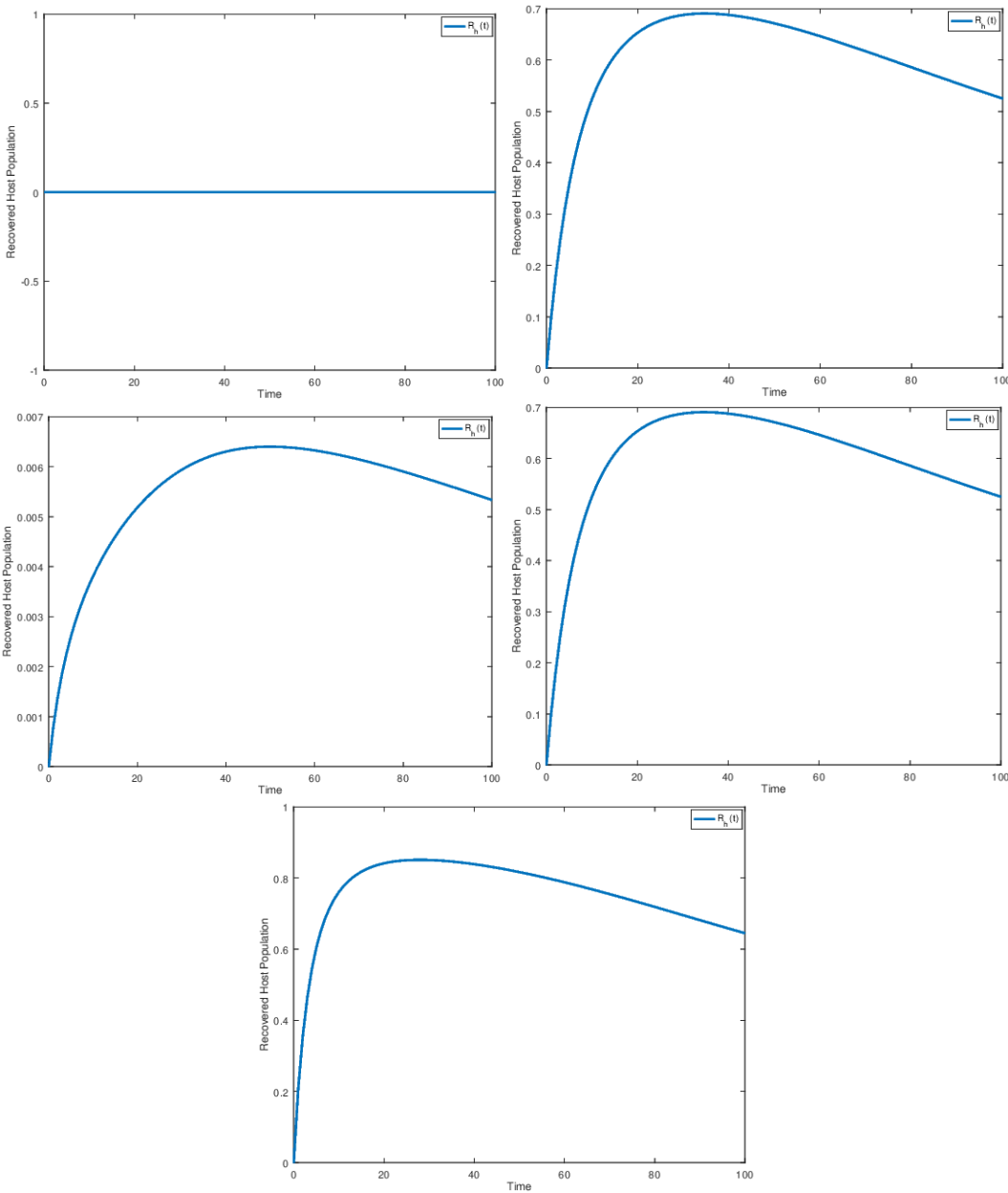
Figure 4: Recovery Host Population
