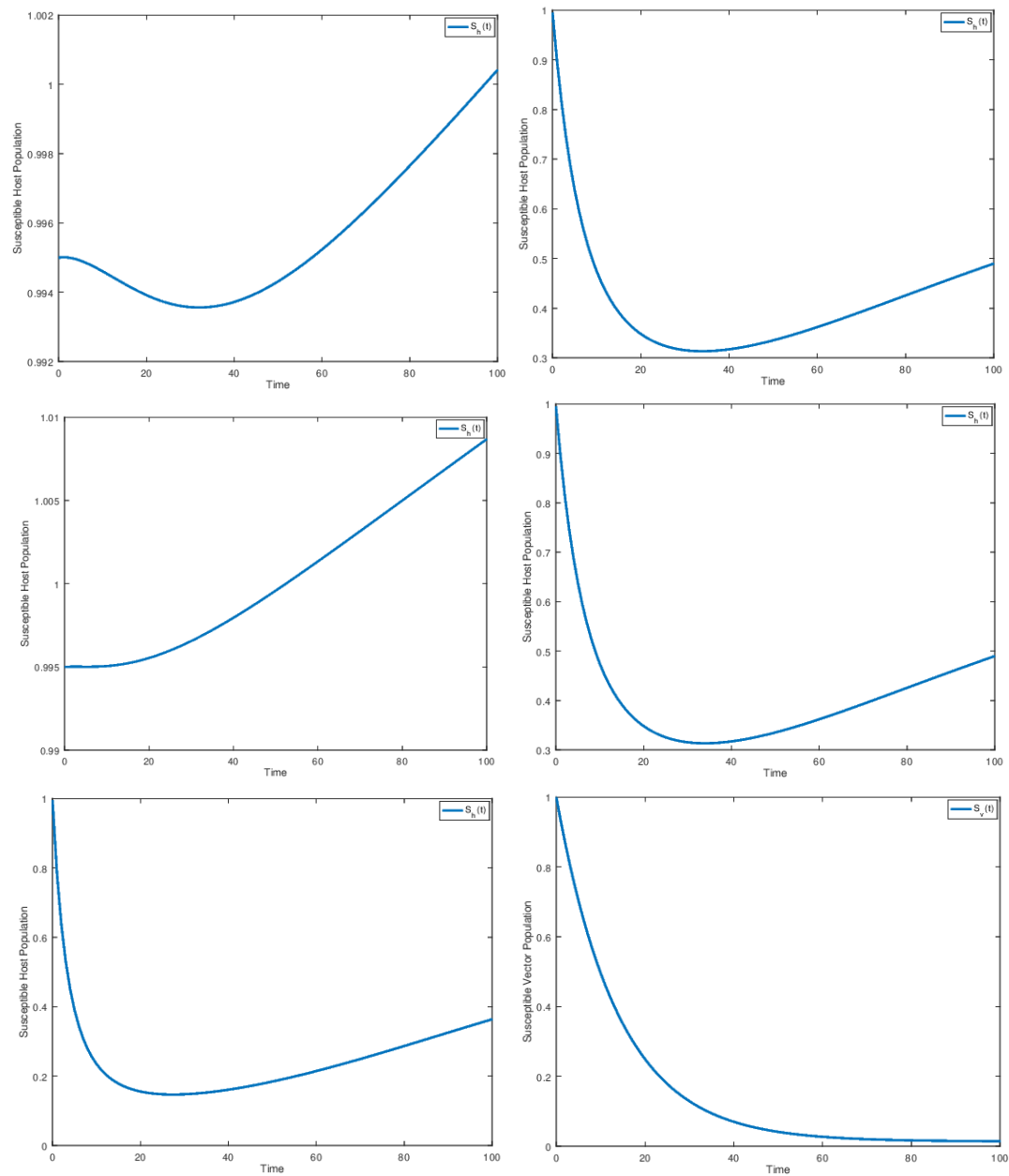
Figure 5: Susceptible Host Population
