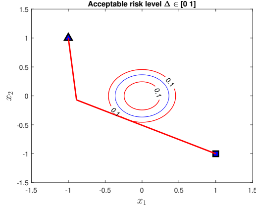
Figure 4: Time-varying SOS optimization with a probability-based static obstacle yields a piece-wise linear trajectory bound by risk.
