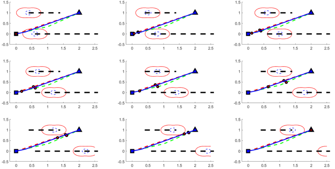
Figure 6: Risk-bound lane-change trajectories for Autonomous vehicle
