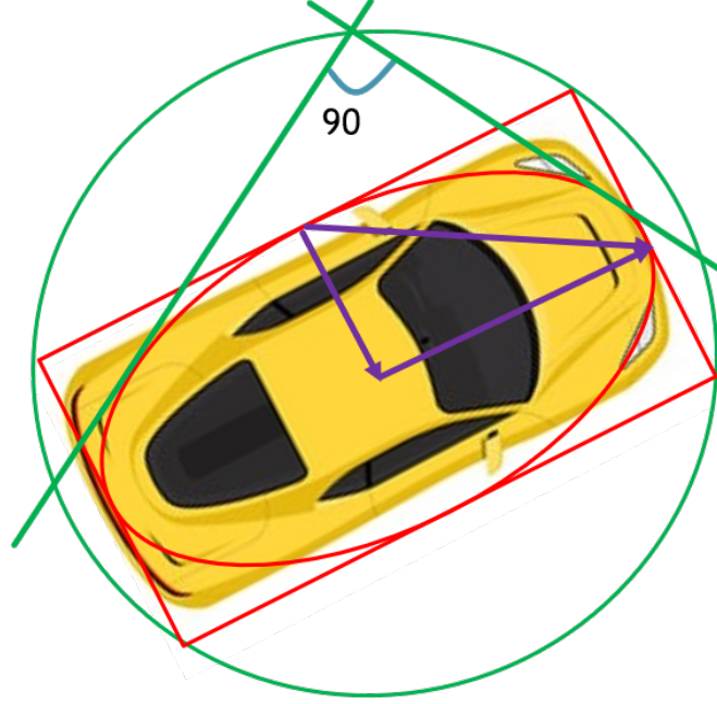
Figure 1: A director circle, an ellipse, and its minimum bounding box
