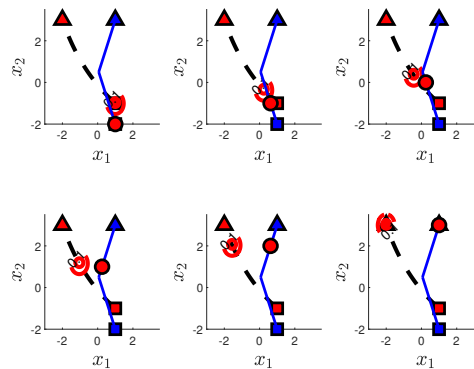
Figure 5: Time-varying SOS optimization with the probabilistic moving obstacle yields a piece-wise linear trajectory subject to risk.
