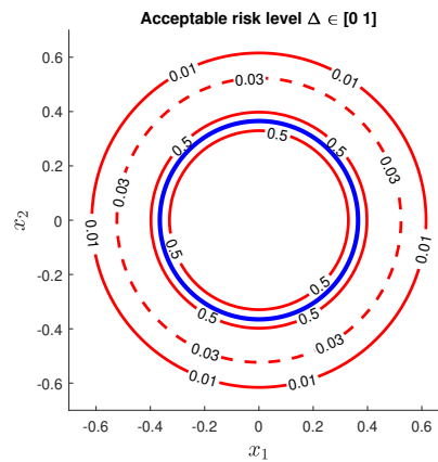
Figure 2: Static \Delta -risk contours as described in (8).
