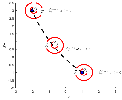
Figure 3: Dynamic \Delta -risk contours as described in (10).
